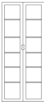
Cabinet F High glass fronted cabinet. h: 210 cm w: 90 cm d: 42 cm
